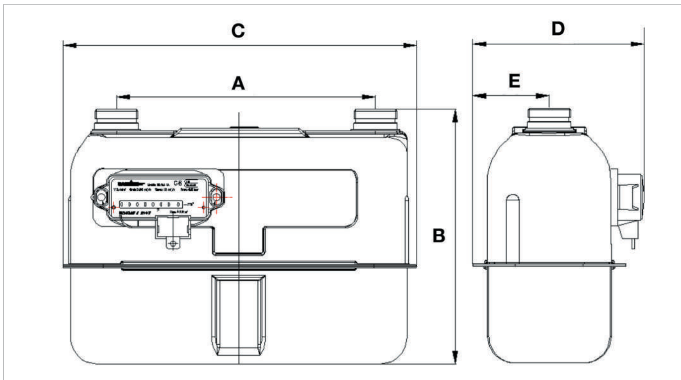
Fig. 6.6. Dimensions RS/2.4
